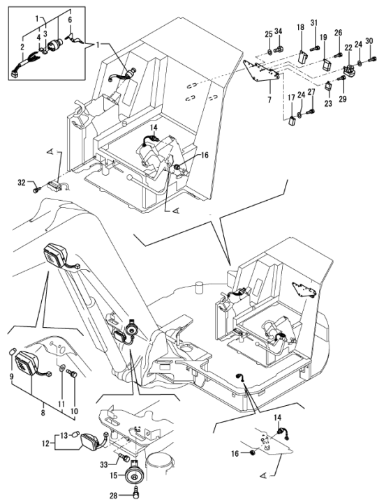
> > SV100 > VEHICLE > Fig. (14) ELECTRIC PART(EQUIPMENT)
