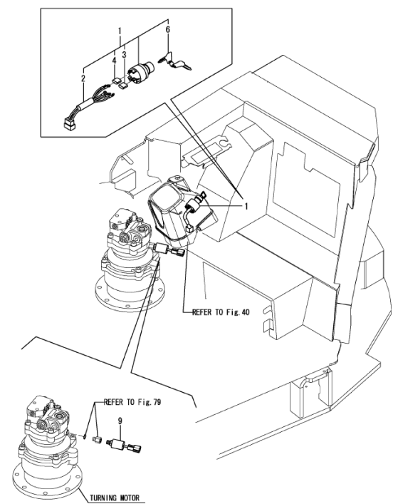
> > SV100-1 > VEHICLE > Fig. (15) ELECTRIC PART(STARTING SWITCH)
