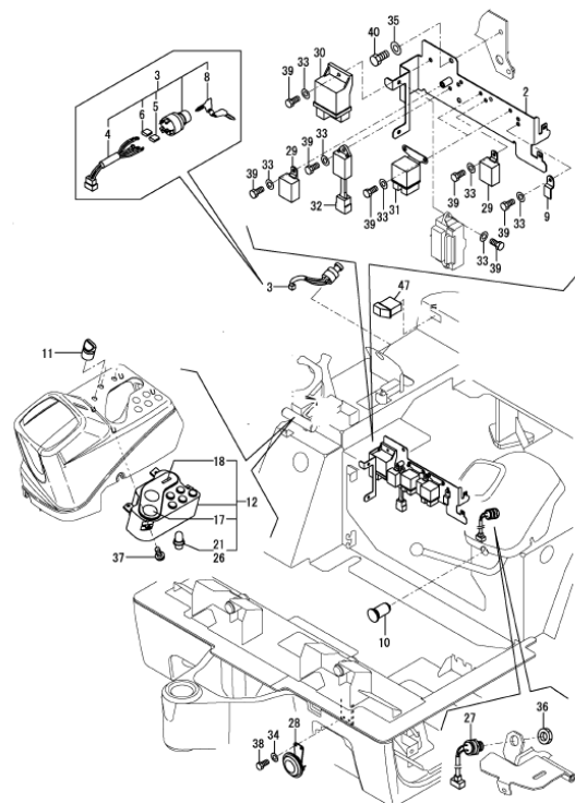
> > SV17E > VEHICLE > Fig. (10) ELECTRIC PART(EQUIPMENT)
