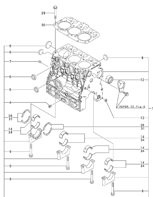
> > SV17 > 3TNV70-VBVA > Fig. (1) CYLINDER BLOCK
