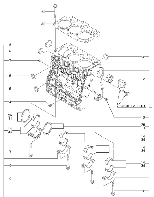
> > SV15 > 3TNV70-XBVA1 > Fig. (1) CYLINDER BLOCK
